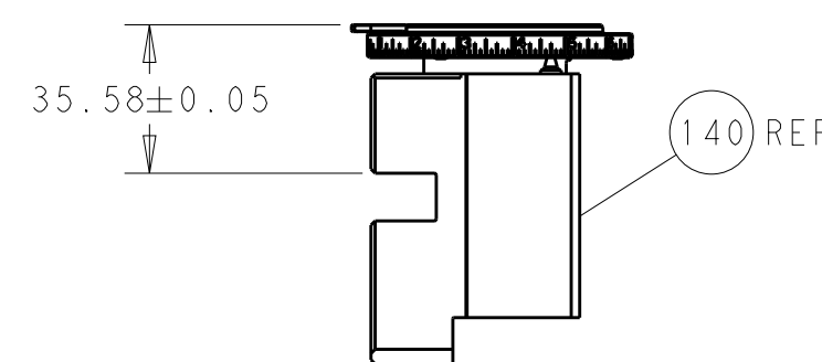
RAM SET-UP
