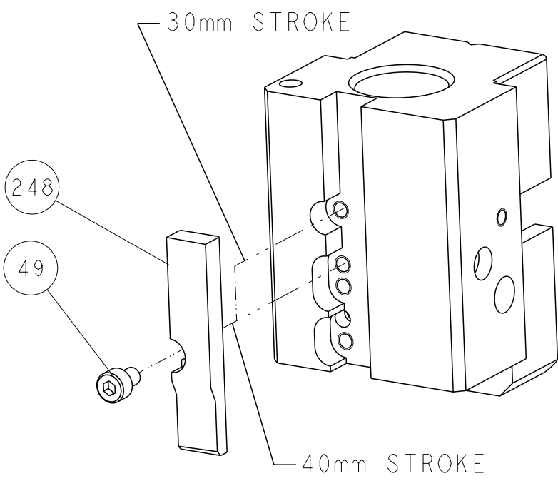
AIR FEED
