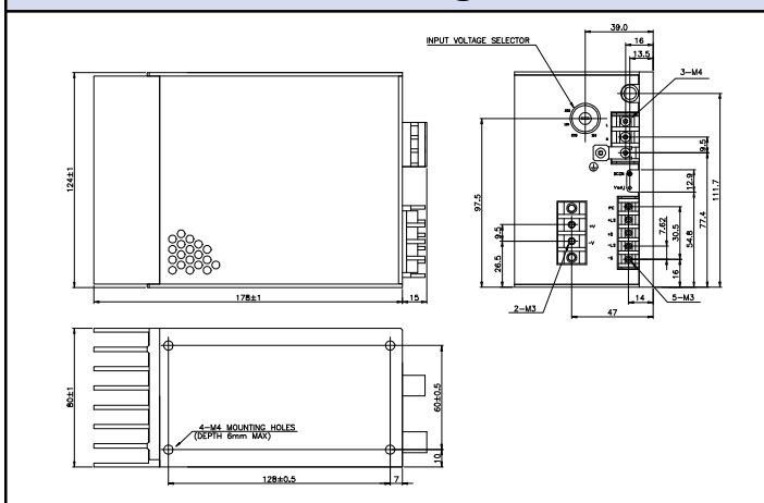
NNS30 Outline Drawing
