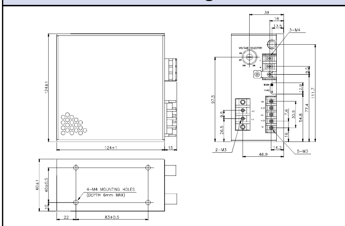
NNS15 Outline Drawing
