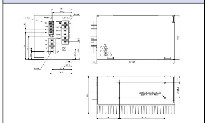
NNS50 Outline Drawing
