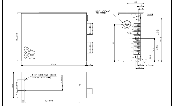
NND15 Outline Drawing
