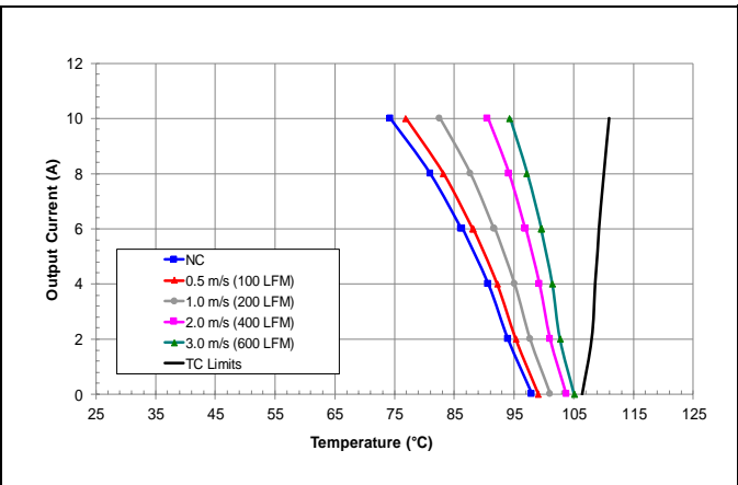
Vo=12V, Vin=24V preliminary maximum output current vs. ambient temperature at nominal input voltage for natural convection (60lfm) to 600lfm with airflow from pin 8 to pin 4.
