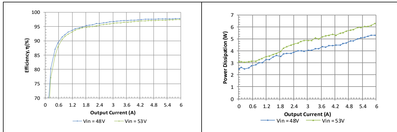
Typical Efficiency and Power Loss vs. Input Voltage
