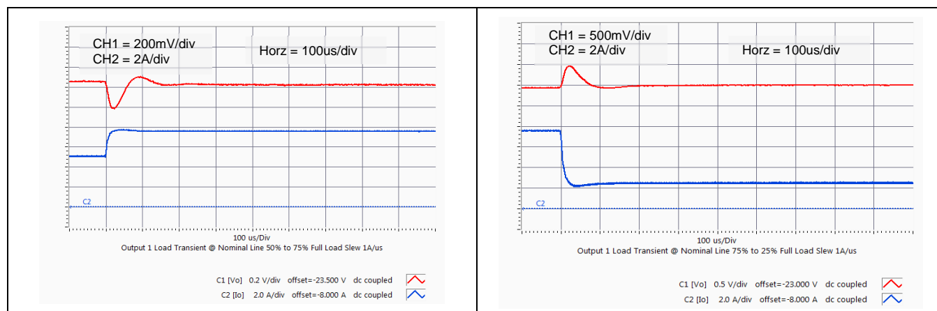
Vo=24V Typical output voltage transient response to load step from 50% to 75% of full load with output current slew rate of 1A/uS. (Cext = 22uF).
