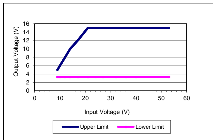
Output Voltage versus Input Voltage Operating Range
