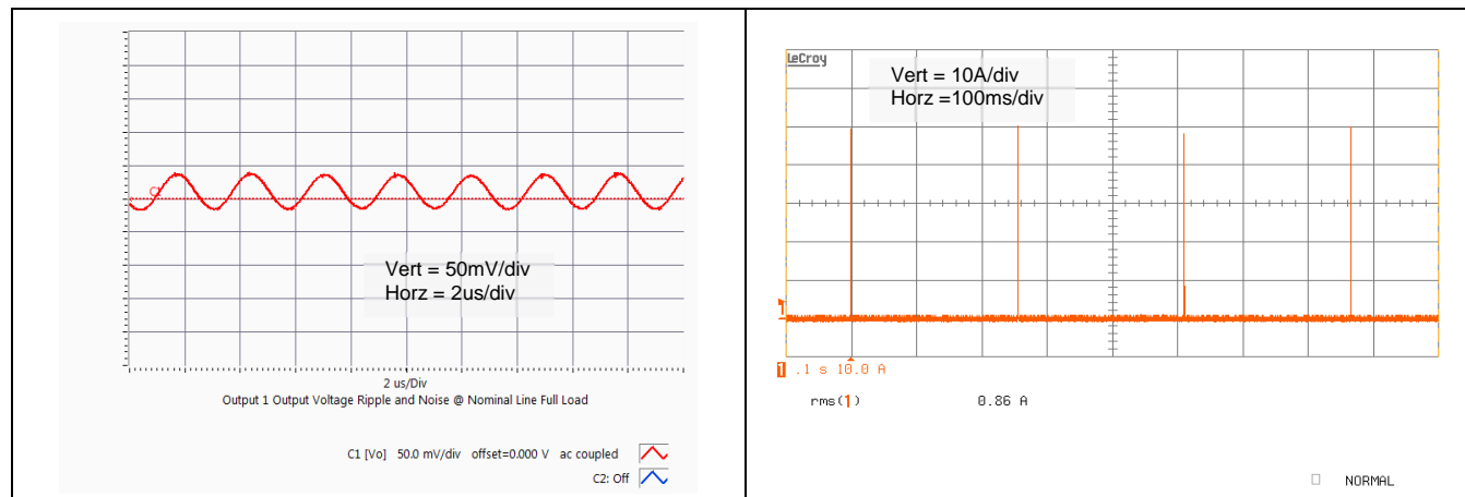
Vo=24V Typical Output Ripple at nominal Input voltage and full load at Ta=25 degrees
