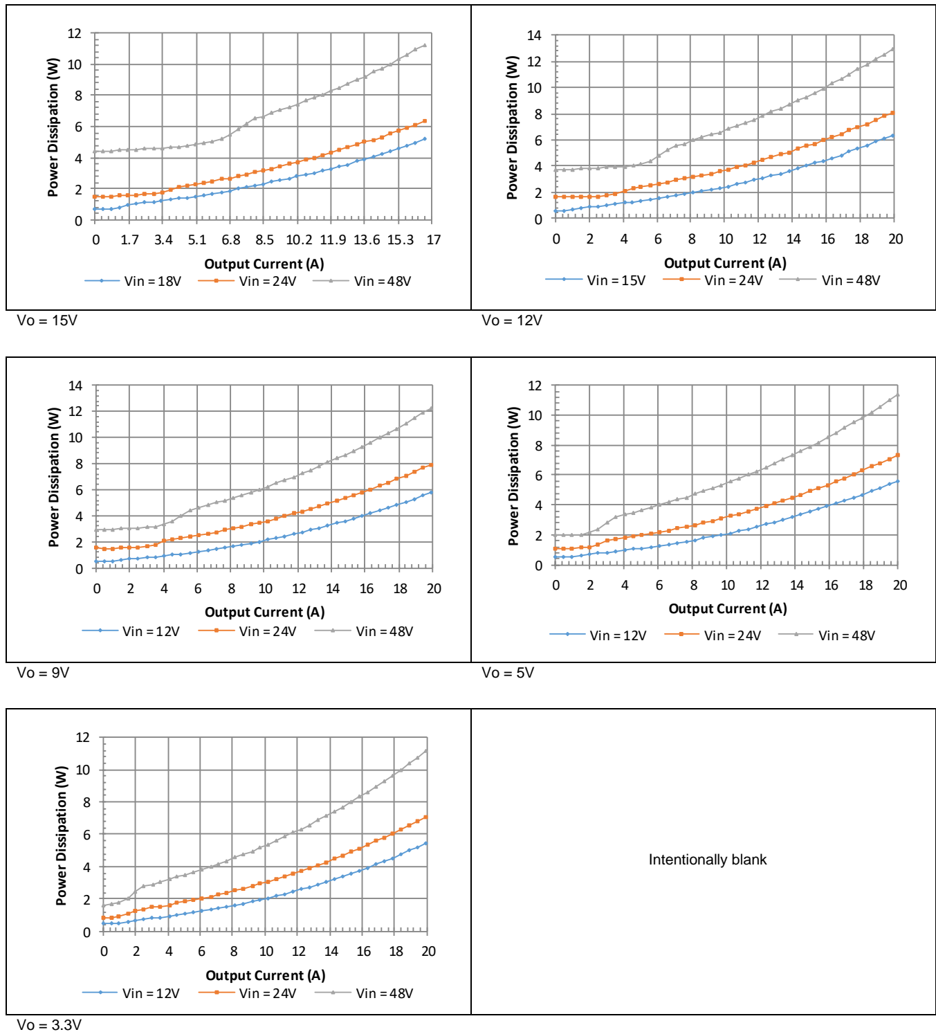
Typical Power Dissipation vs. Input Voltage
