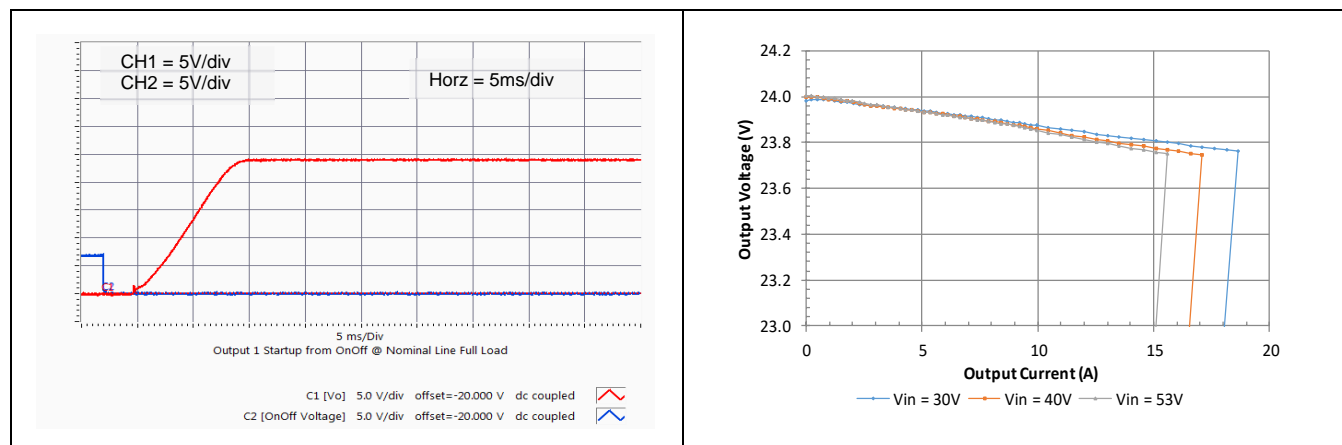
Vo=24V Typical startup characteristic from on/off at full load. Ch1 - output voltage, Ch2 – on/off signal
