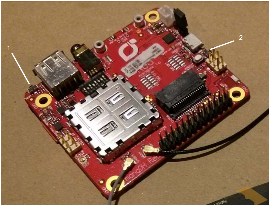
Figure 3-23: Reset Switches
