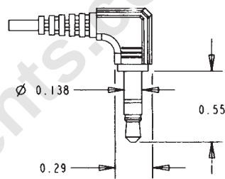
END CODE: 36 3.5 mm RIGHT-ANGLE PLUG
