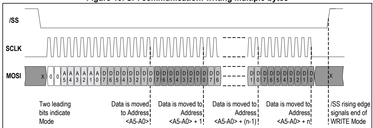
Figure 10. SPI communication: writing multiple bytes
