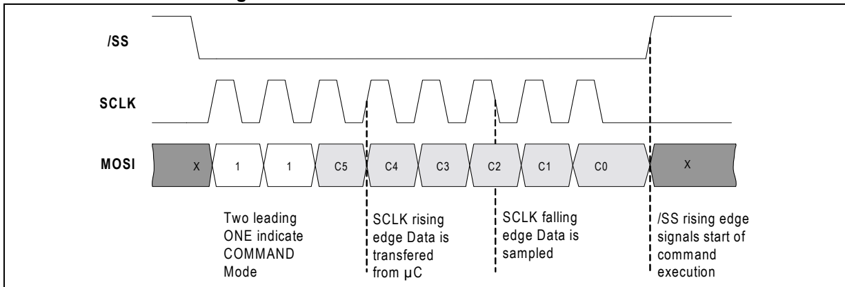
Figure 14. SPI communication: direct command
