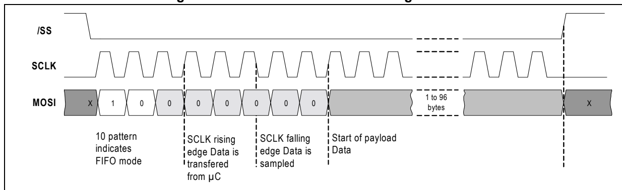
Figure 12. SPI communication: loading of FIFO
