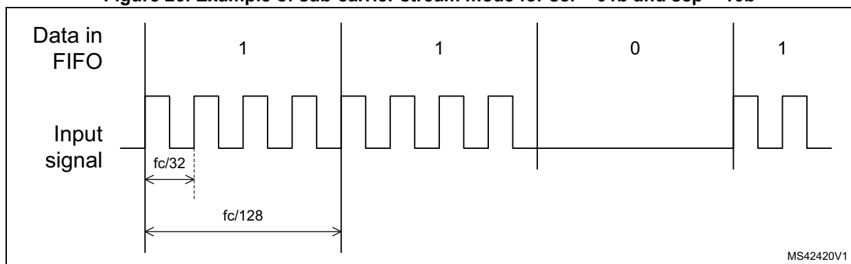
Figure 26. Example of sub-carrier stream mode for scf = 01b and scp = 10b
