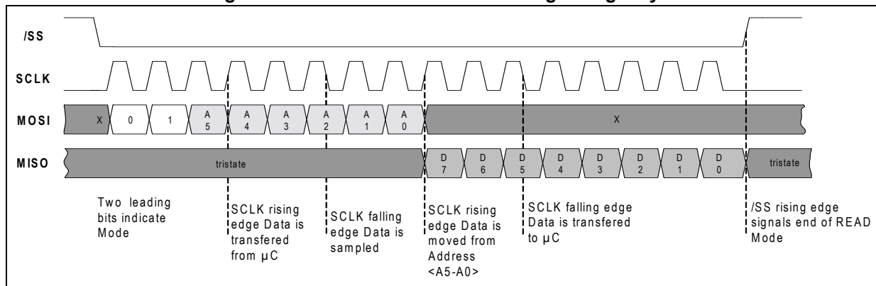
Figure 11. SPI communication: reading a single byte
