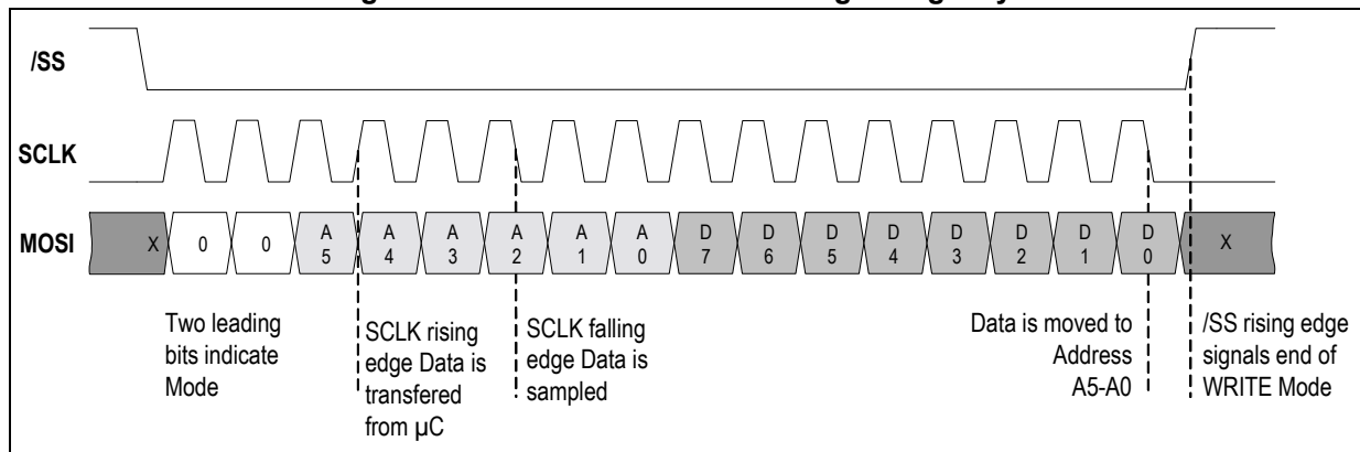
Figure 9. SPI communication: writing a single byte
