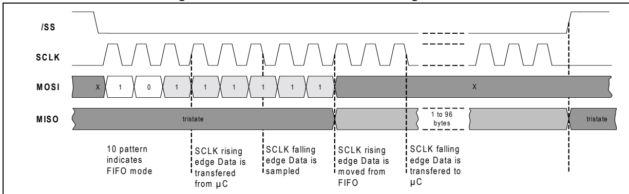
Figure 13. SPI communication: reading of FIFO
