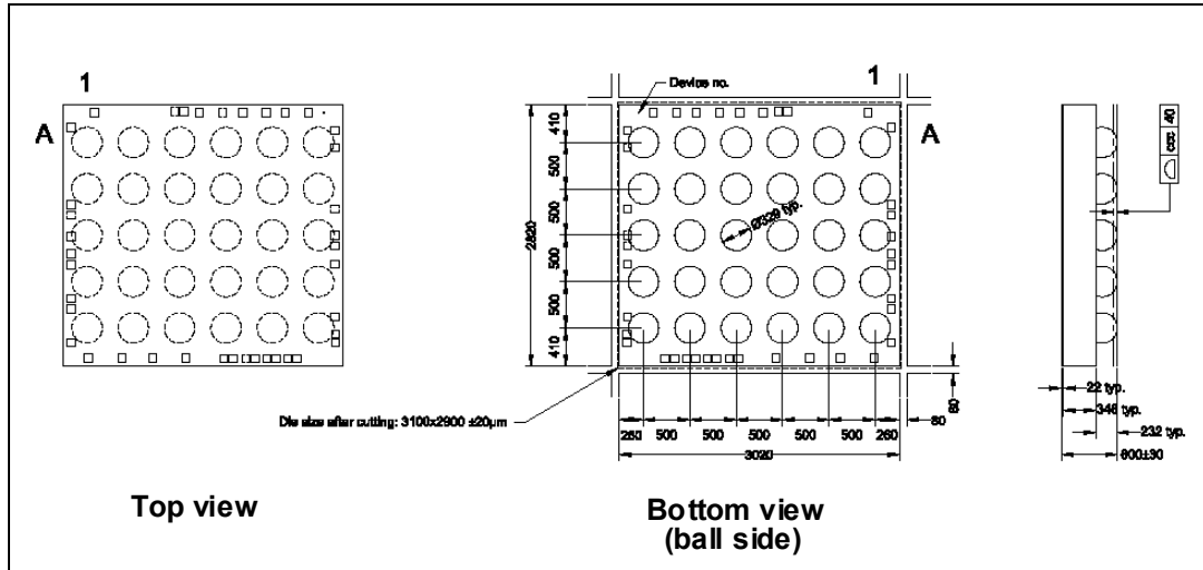
Figure 34. WLCSP package outline
