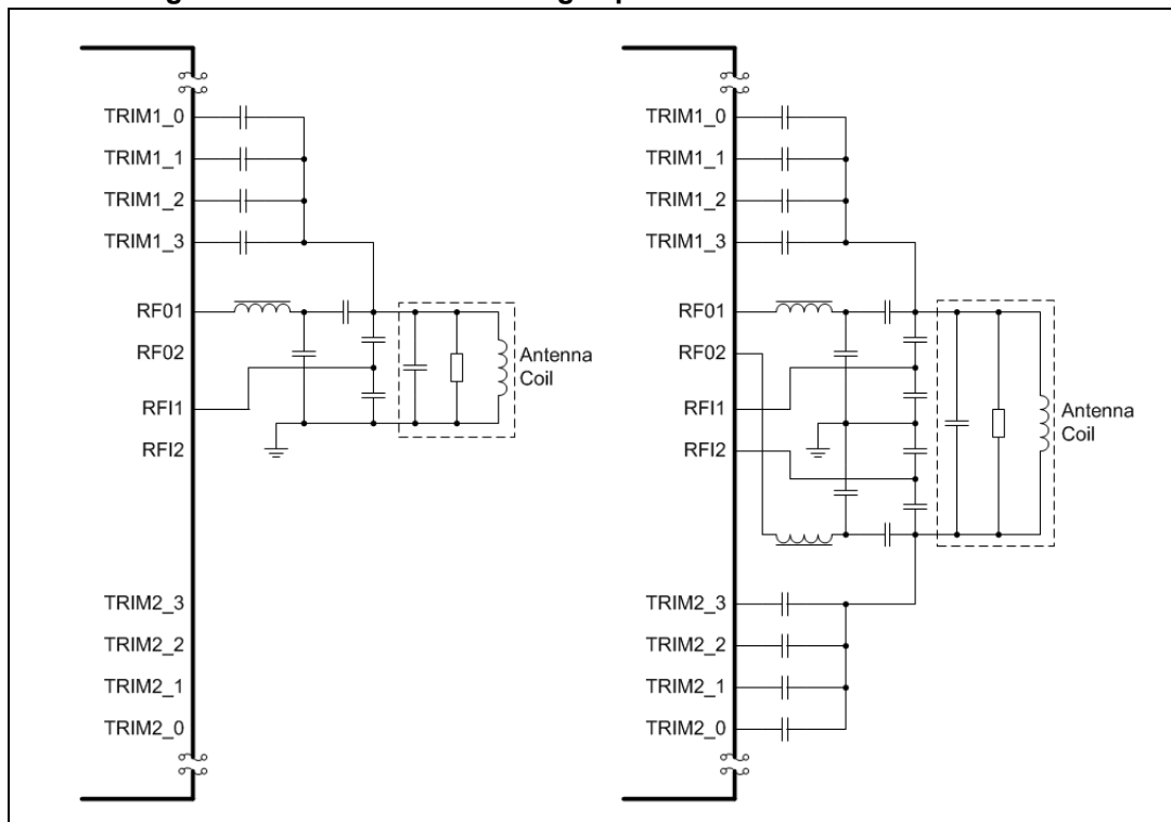
Figure 25. Connection of tuning capacitors to the antenna LC tank
