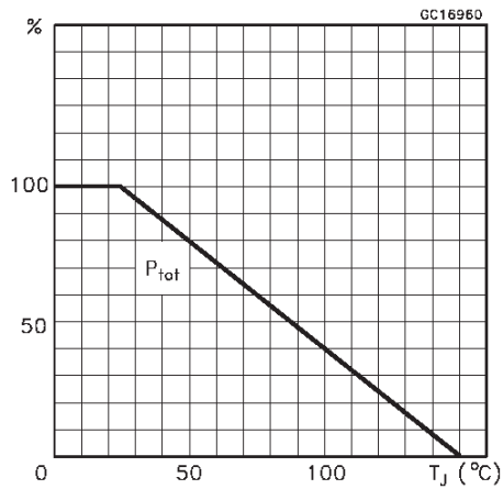
Derating Curve
