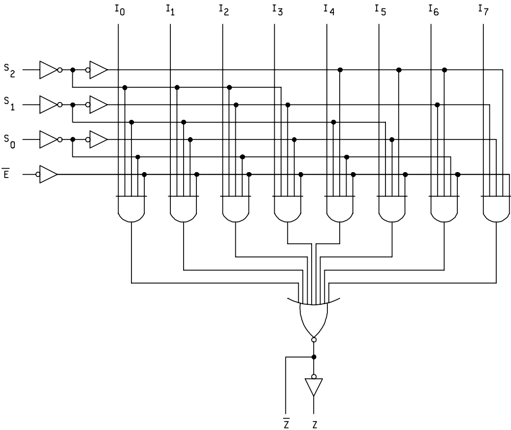
FIGURE 3. Logic diagram.
