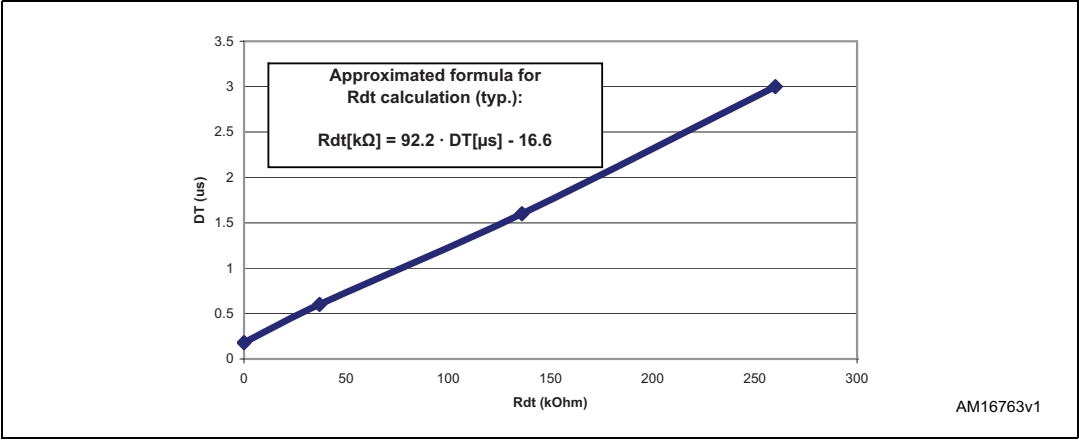
Figure 4. Typical deadtime vs. DT resistor value
