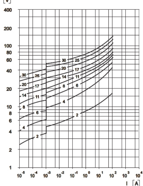
Model Size 0805
