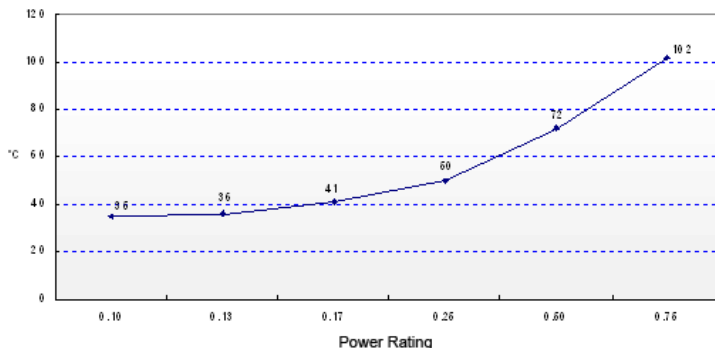
CSR1206 100m Surface Temp Rise
