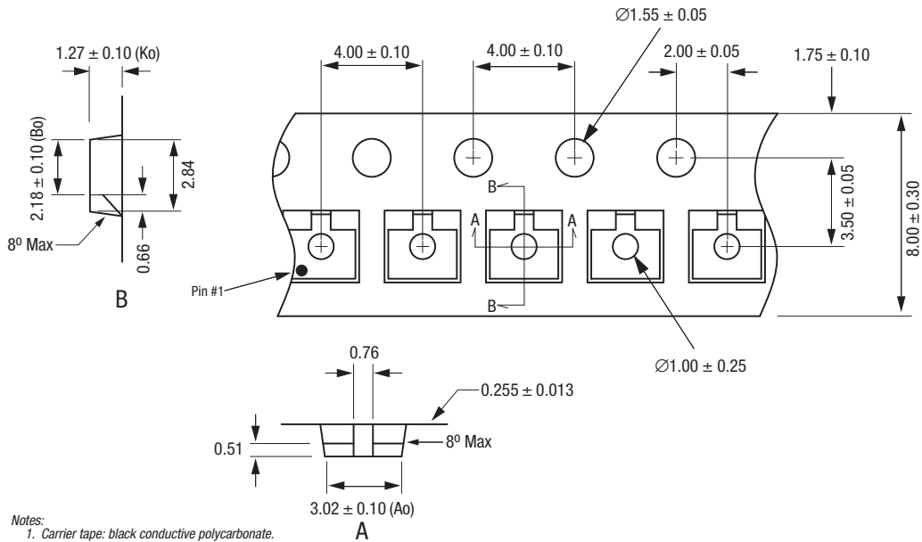
Figure 10. SOT-23 Tape and Reel Dimensions
