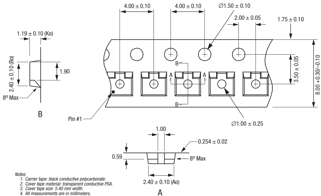
Figure 6. SC-70 Tape and Reel Dimensions
