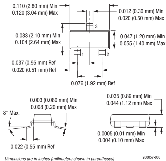
Figure 8. SOT-23 Package Dimensions
