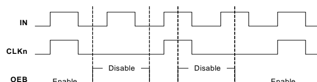
Figure 3. OEB Glitchless Operation
