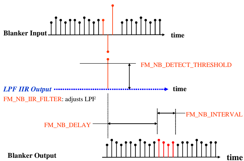
Figure 7. FM Noise Blanker
