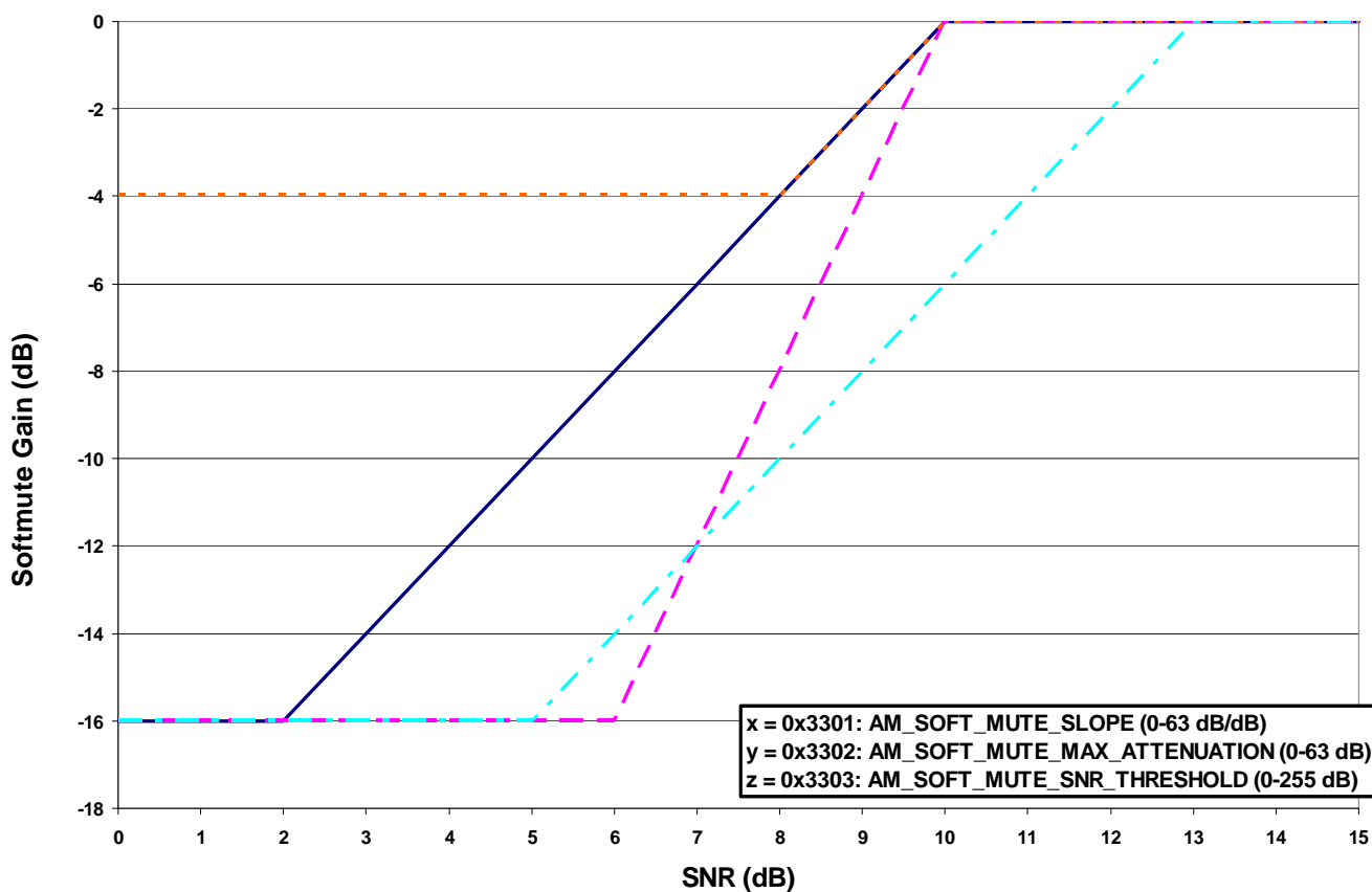
Figure 13. AM Softmute SNR
