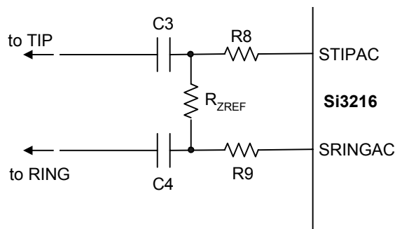
Figure 25. R 7REF External Resistor Placement
