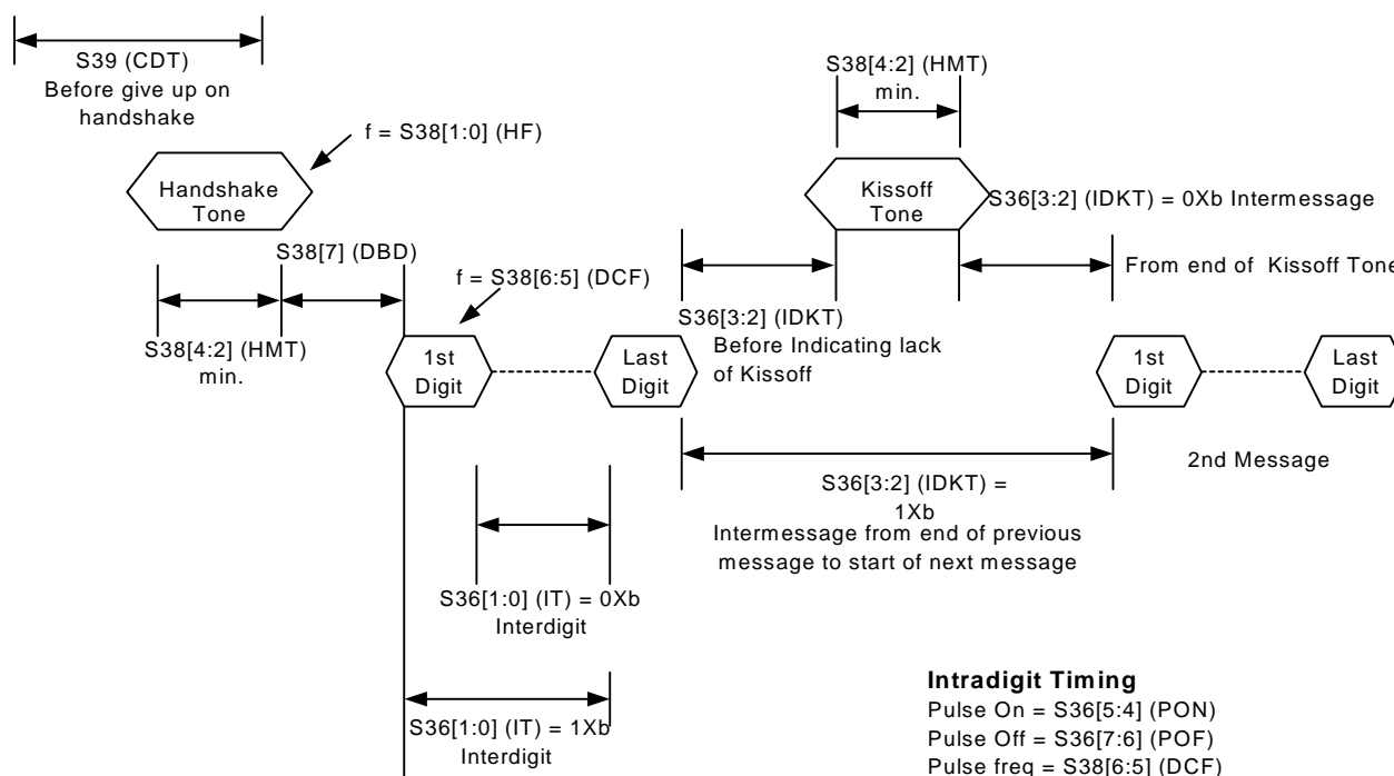
Figure 12. !7 Security Timing
