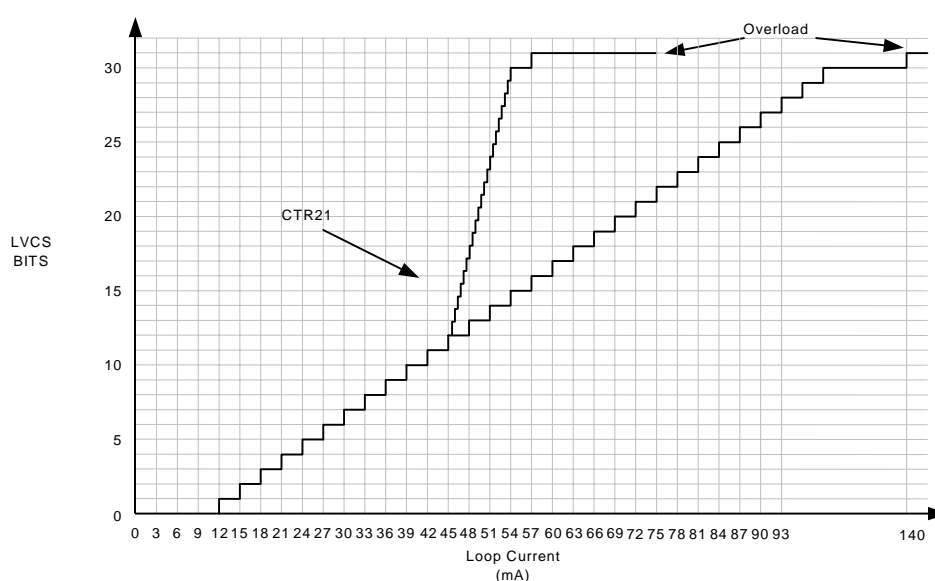
Figure 8. Loop Current—LVCS Transfer Function
