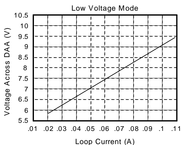
Figure 17. Low Voltage Mode I/V Characteristics
