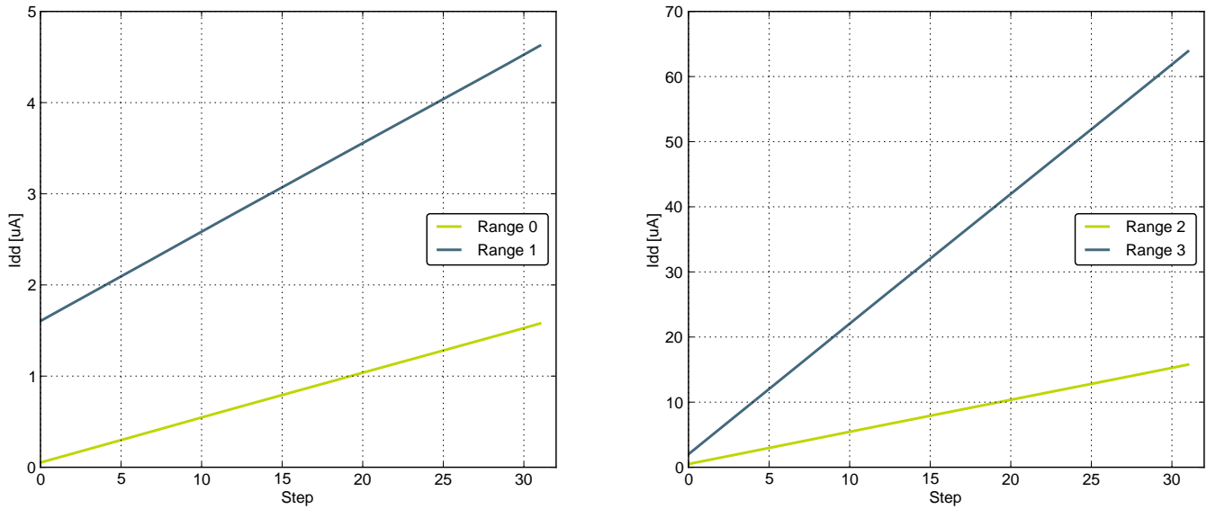
Figure 4.36. IDAC Linearity
