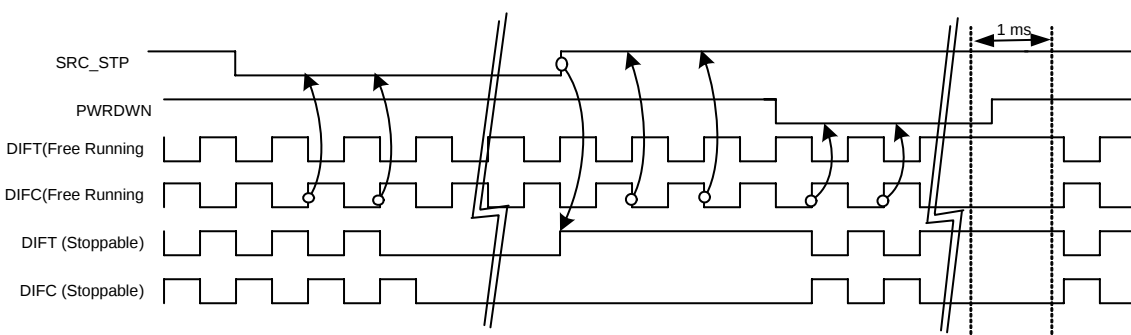
Figure 7. SRC_STP = Tri-state, PWRDWN = Driven, OE_INV = 0
