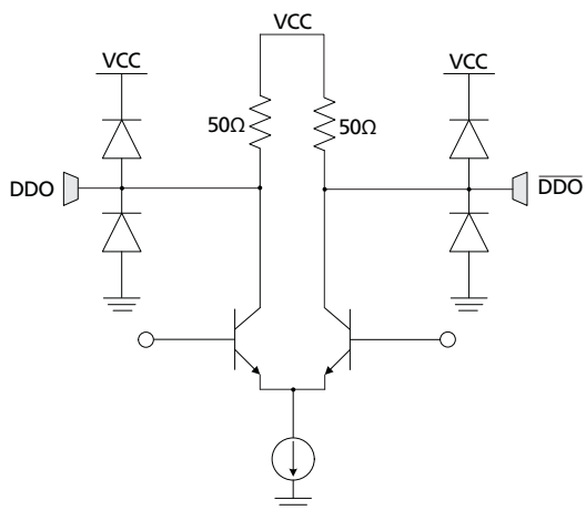
Figure 3-5: High-speed Outputs ( \overline{\text{DDO1/RCO}} , \overline{\text{DDO1/RCO}} , \overline{\text{DDO0}} , \overline{\text{DDO0}} )
