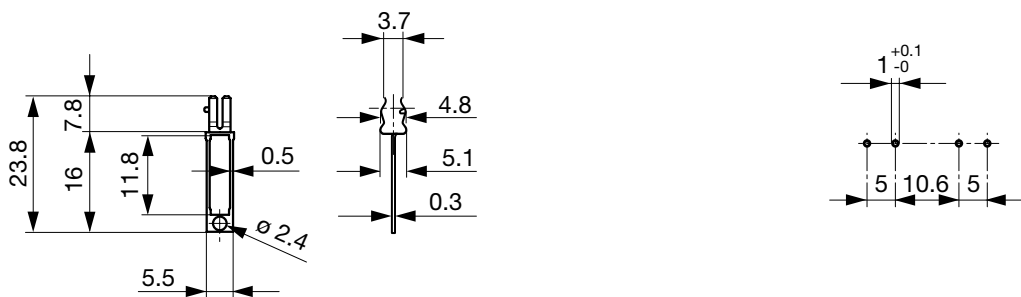
Drilling diagram
