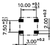
J-lead
