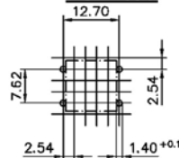
PCB lead
