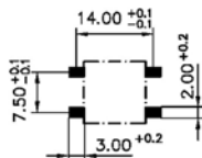
Gullwing lead
