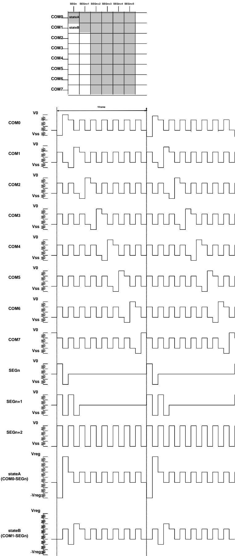
Figure 10. Wave form of line inversion
