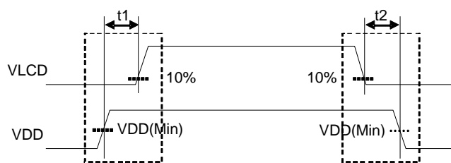
Figure 14. Recommended Power ON/OFF Sequence
