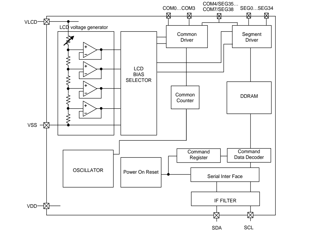
Figure 2. Block Diagram
