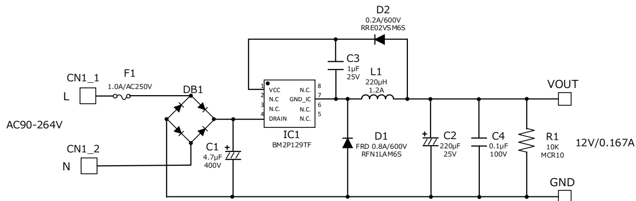
Figure 23. BM2P129TF-EVK-001 Schematics
