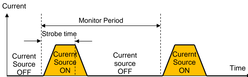
Figure 13. Intermittent Monitoring
