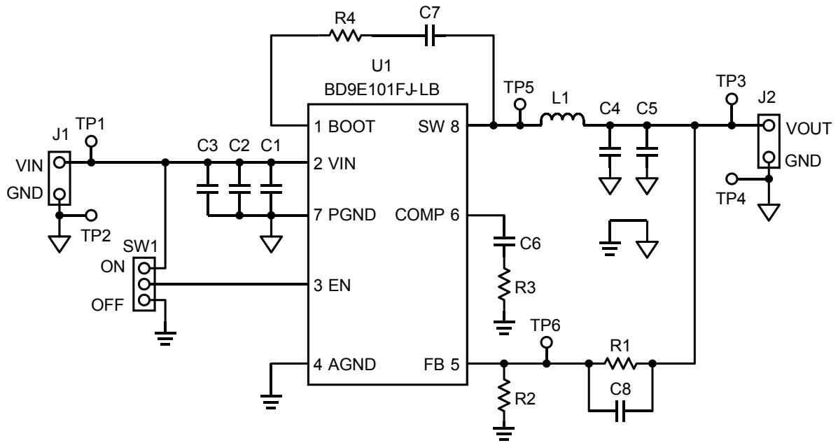
Figure 2. BD9E101FJ-EVK-001 Circuit Diagram
