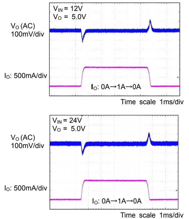
Figure 12. Load Transient Characteristics
