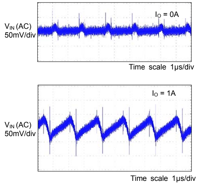
Figure 16. Input Voltage Ripple Wave V_{IN} = 12V, V_O = 5.0V
