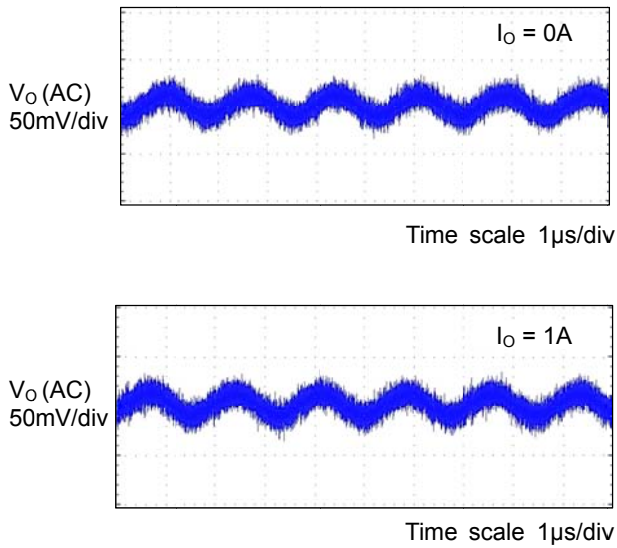
Figure 17. Output Voltage Ripple Wave V_{IN} = 12V, V_O = 5.0V
