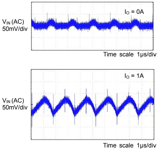
Figure 15. Input Voltage Ripple Wave V_{IN} = 12V, V_O = 5.0V
