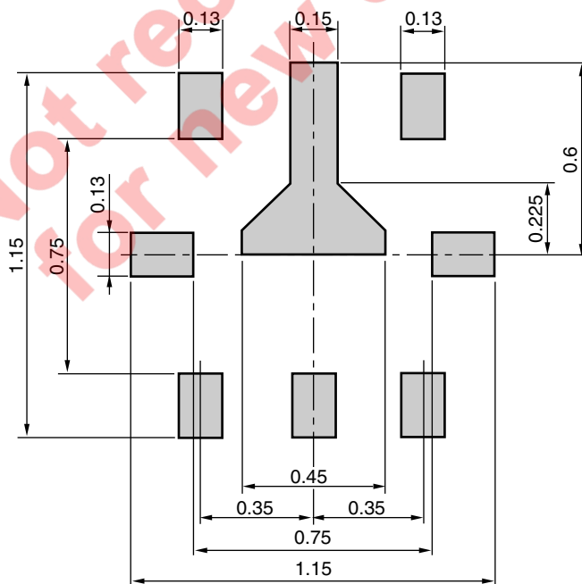
SOLDER MASK
