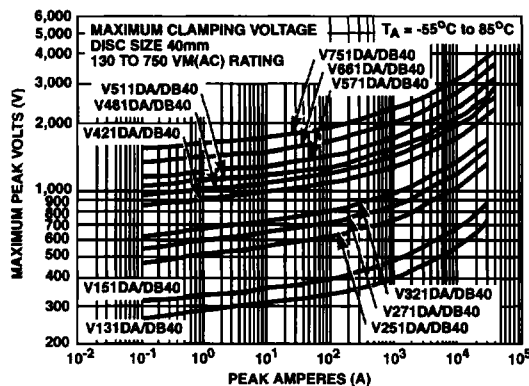
FIGURE 3. CLAMPING VOLTAGE FOR V131DA40, V131DB40 - V751DA40, V751DB40
