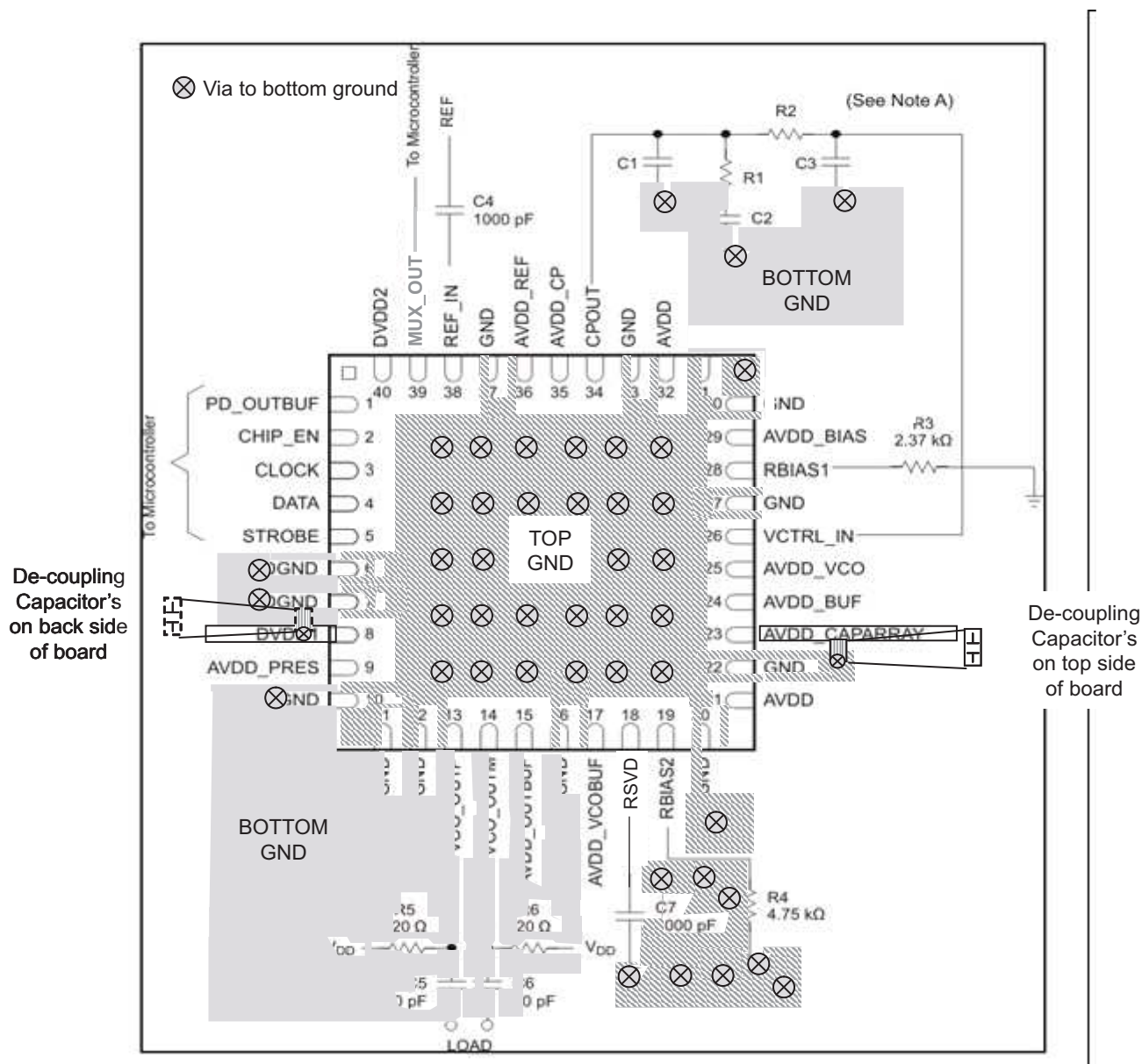
Figure 18. TRF3762 Layout
