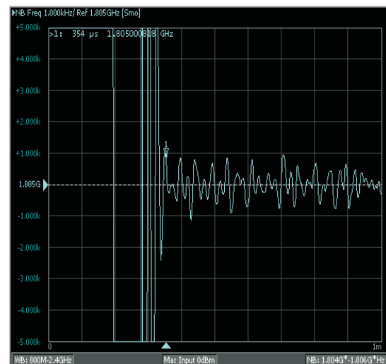
Figure 17. Frequency Locktime
