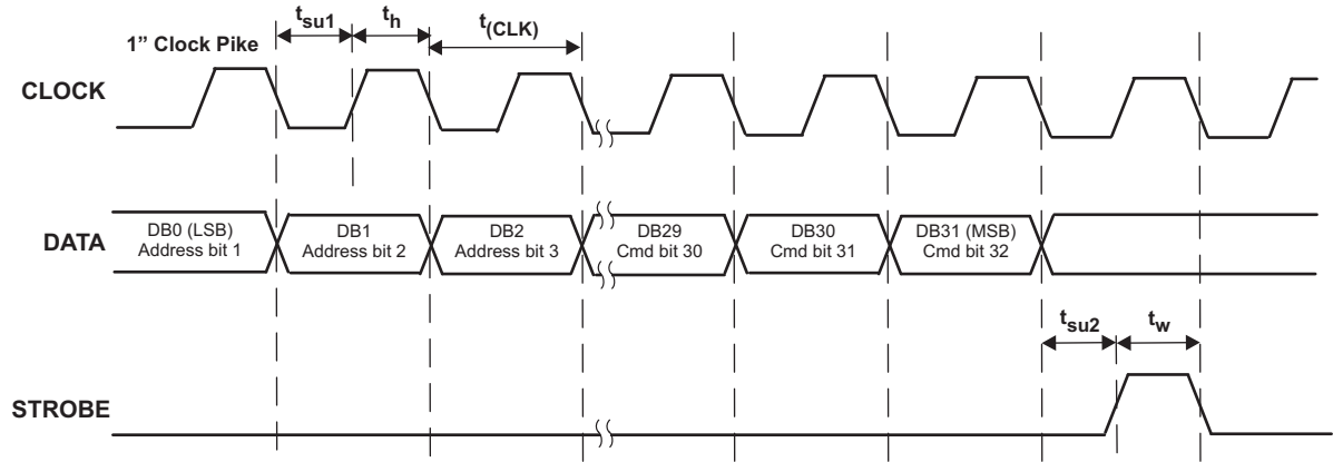
Figure 11. Serial Programming Timing Diagram
