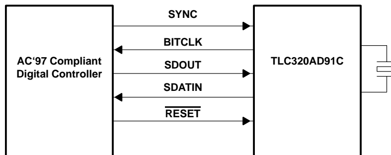
Figure 2–2. AC-Link Signals
