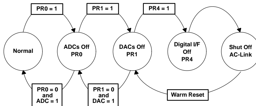
Figure 2–9. TLC320AD91C Power-Down/Power-Up Flow Example With Analog Still Alive
