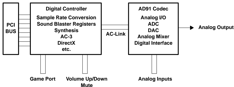
Figure 5–1. System Diagram
