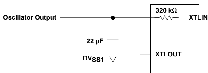
Figure 2–6. External Oscillator Configuration
