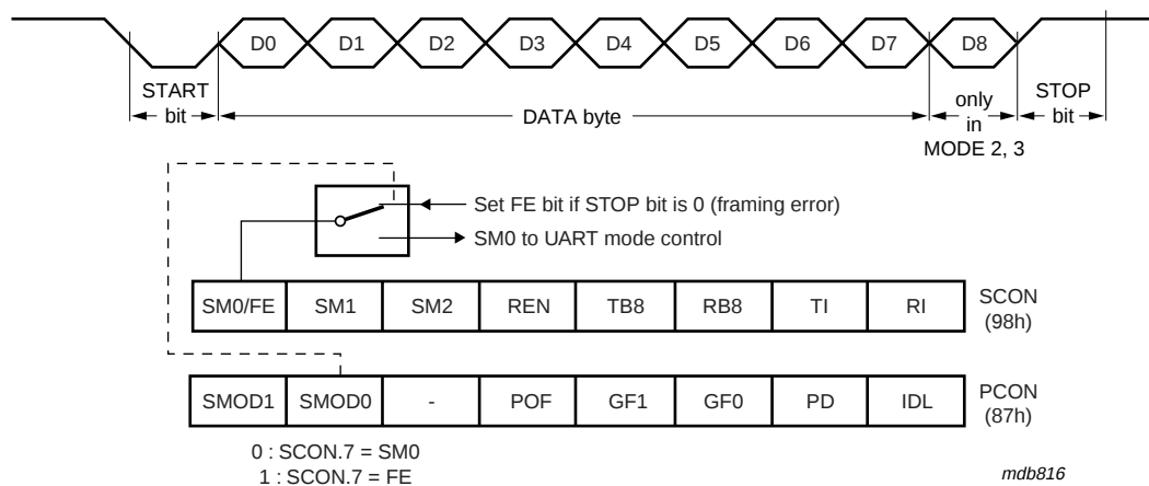
Fig 6. UART framing error detection
