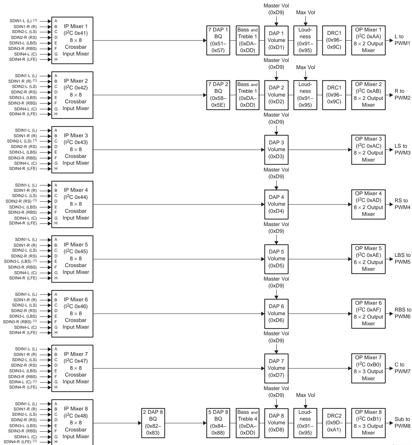
Figure 2-2. TAS5508A Architecture With I²C Registers ( f_s = 176.4 kHz or f_s = 192 kHz)
