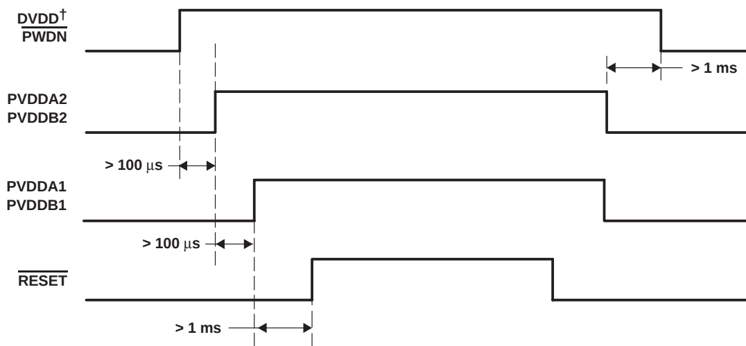
Figure 3. Power-Up/Power-Down Sequence
