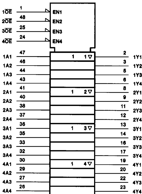
logic symbol†
