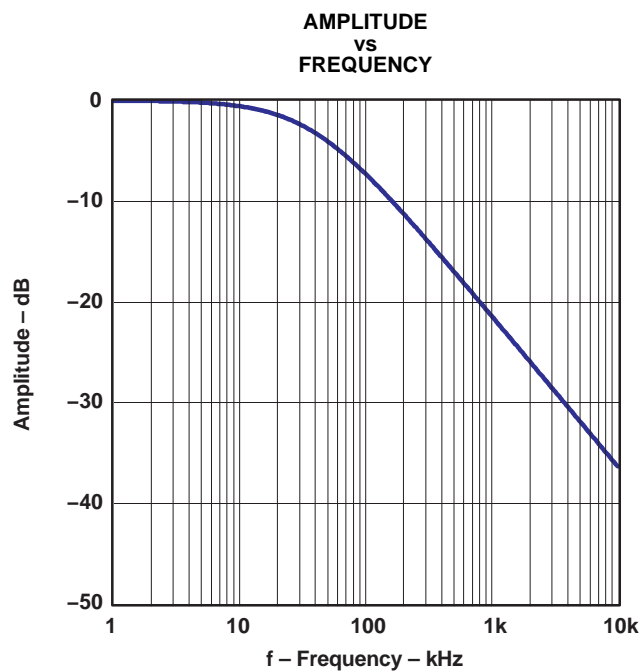
Figure 22. Stop-Band Characteristic
