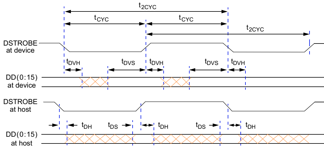
Figure 16 Timing Diagram—Sustained Ultra DMA Data In Burst
