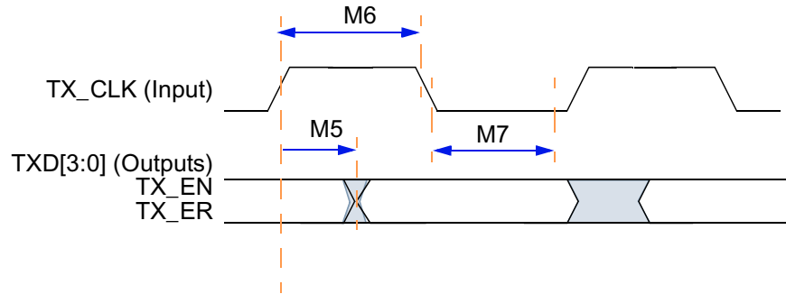
Figure 27 Ethernet Timing Diagram—MII Tx Signal
