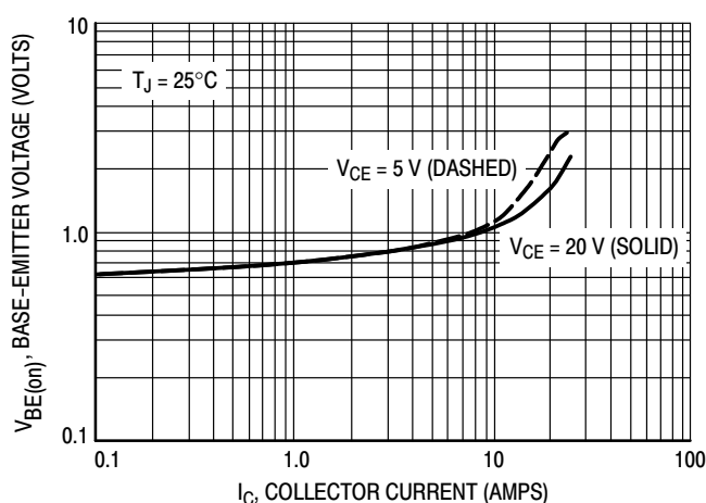
Figure 8. Typical Base-Emitter Voltage
