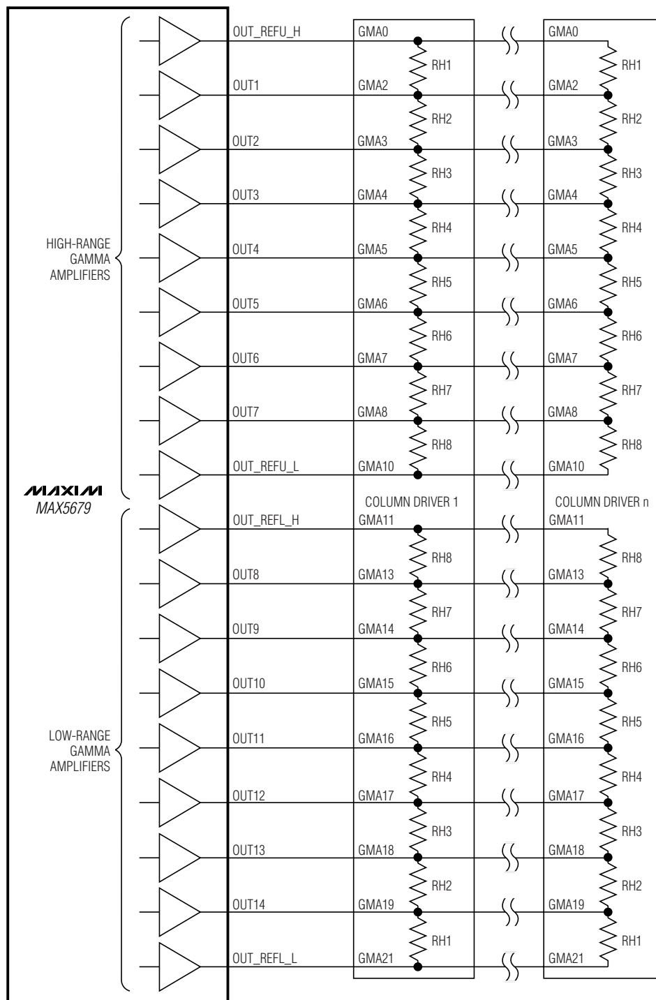
Figure 10. Typical LCD Application
