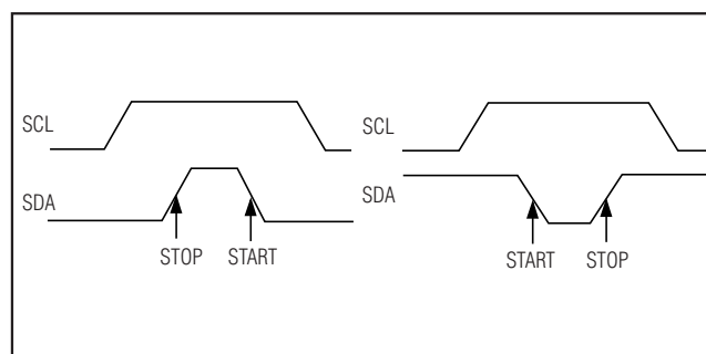
Figure 3. Valid START/STOP Conditions
