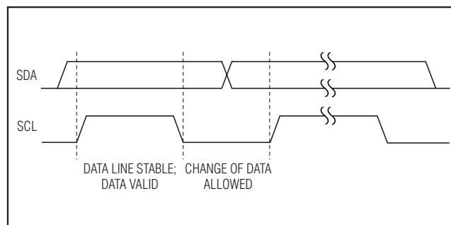
Figure 4. Bit Transfer
