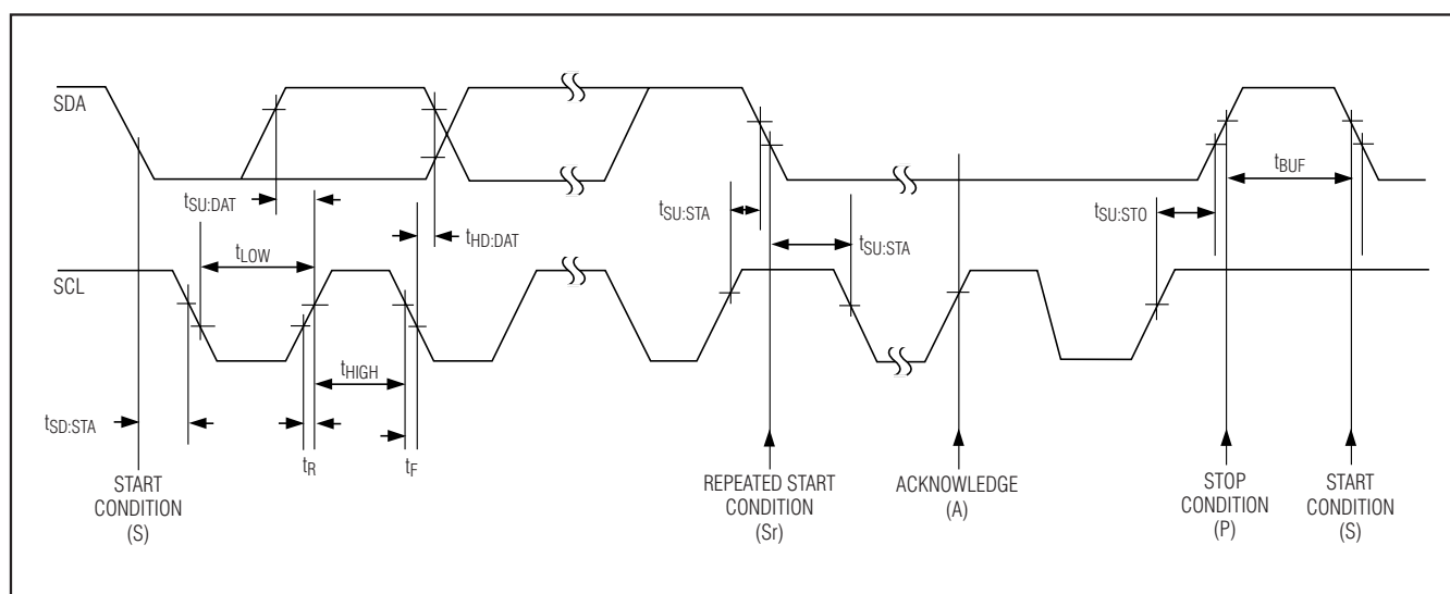
Figure 1. I 2 C 2-Wire Serial-Interface Timing Details
