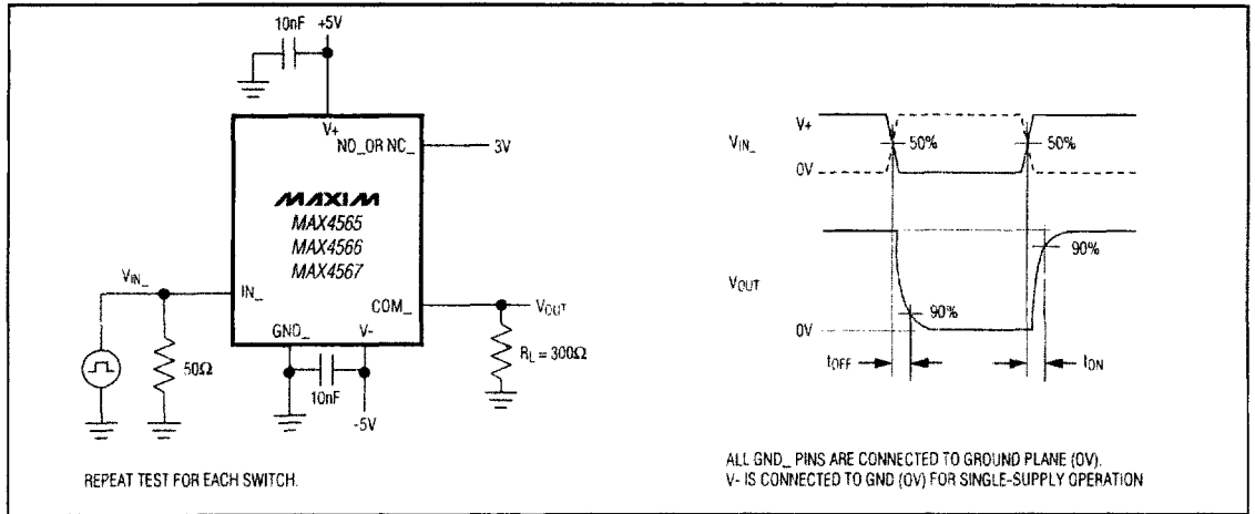
Figure 3. Switching Time
