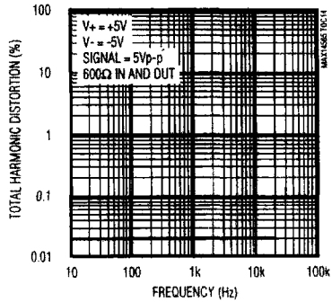
MAX4567 TOTAL HARMONIC DISTORTION vs. FREQUENCY
