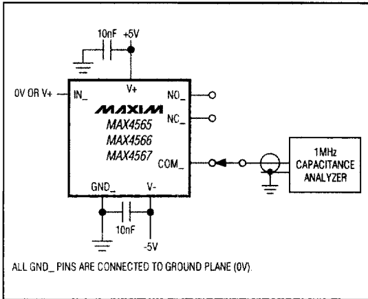
Figure 7. NO_, NC_, COM_ Capacitance
