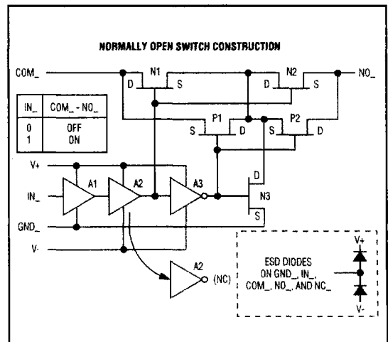
Figure 1. T-Switch Construction
