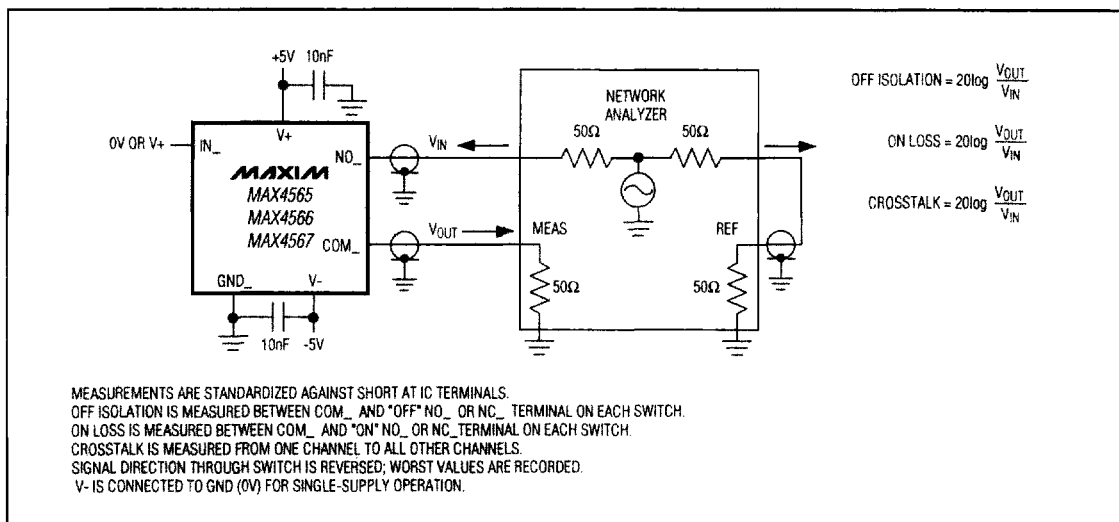
Figure 6. On Loss, Off Isolation, and Crosstalk
