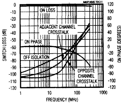
MAX4565 FREQUENCY RESPONSE
