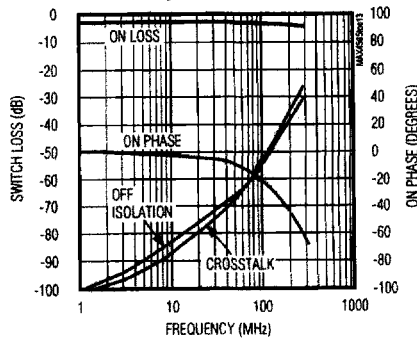
MAX4567 FREQUENCY RESPONSE
