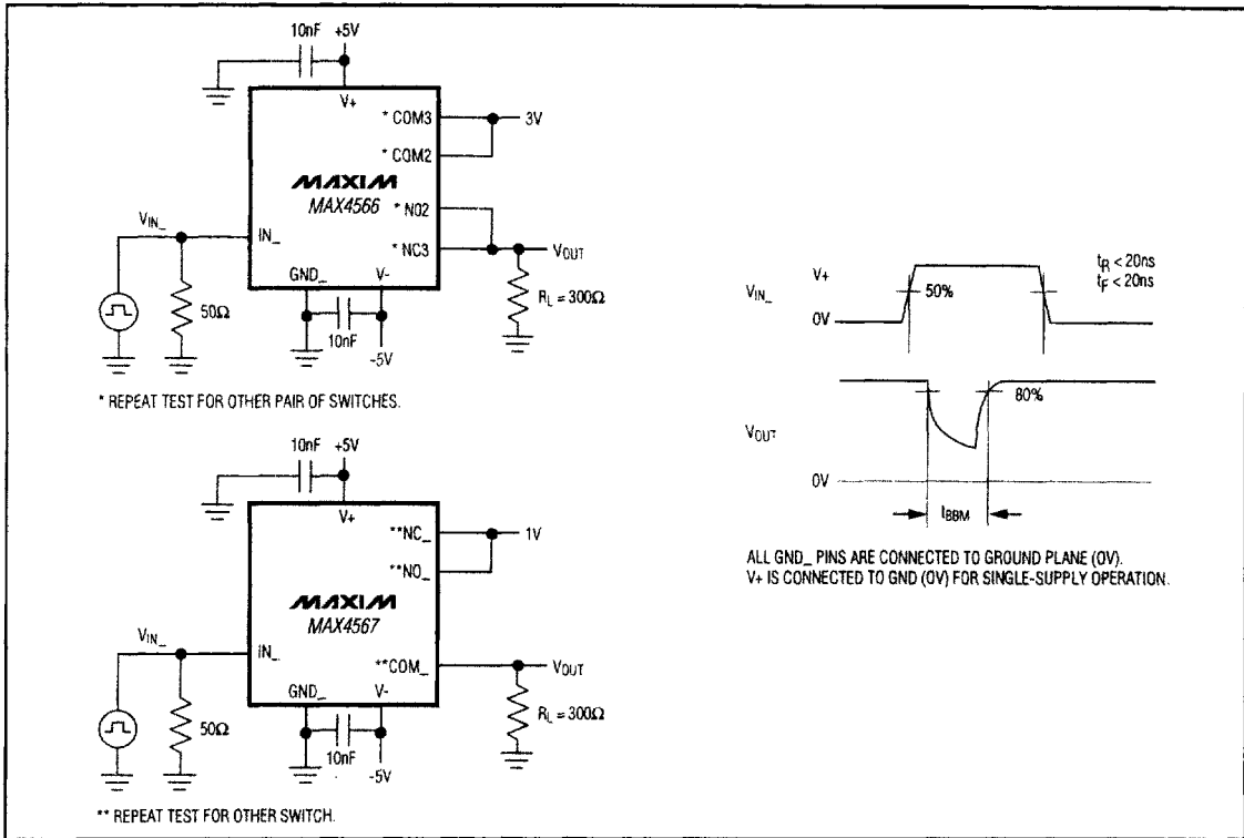
Figure 4. Break-Before-Make Interval (MAX4566/MAX4567 only)
