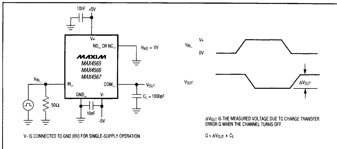
Figure 5. Charge Injection
