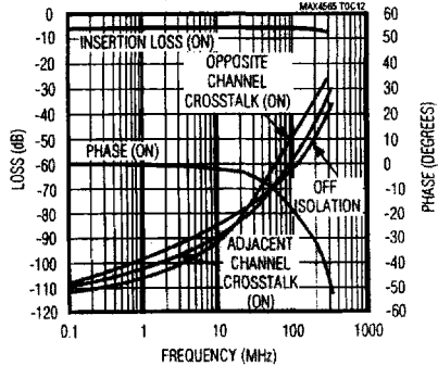
MAX4566 FREQUENCY RESPONSE
