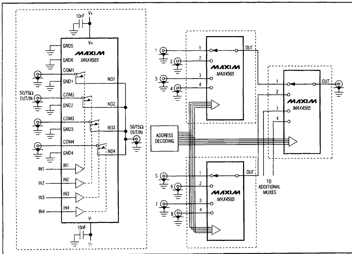
Figure 2. 4-Channel Multiplexer
