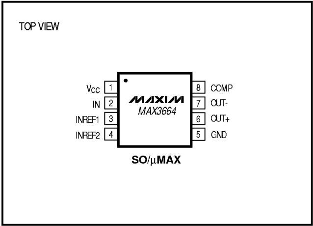
Pin Configuration
