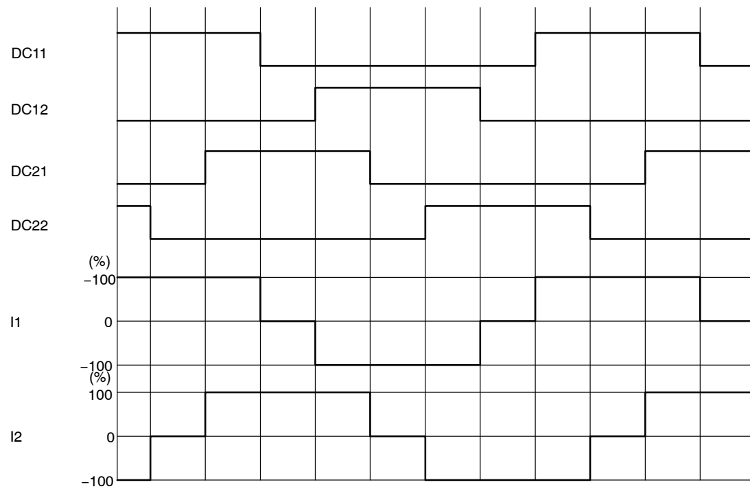
Figure 19. Half Step Full Torque (CW Mode)
