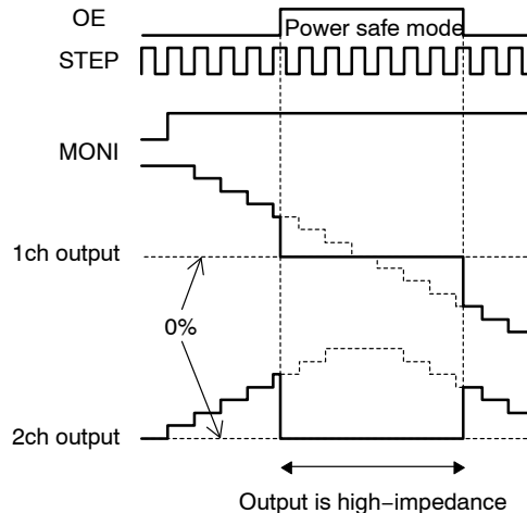
Figure 8. Output Enable Function
