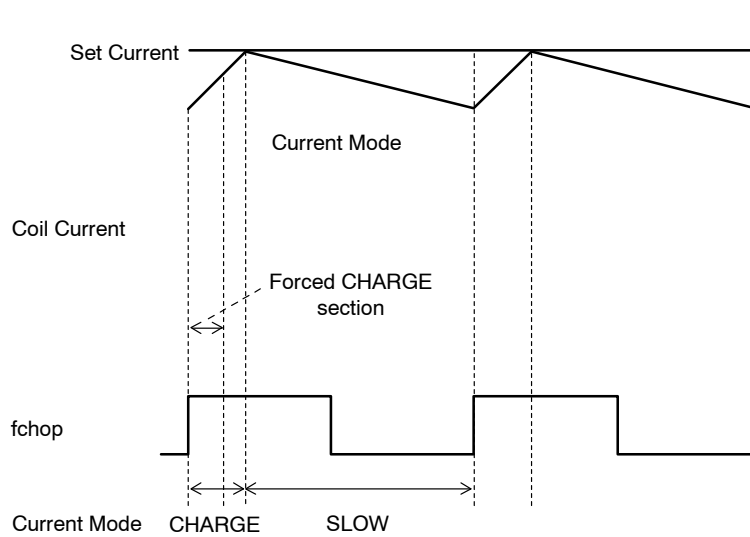
Figure 17. Current Limit Control Time Chart
