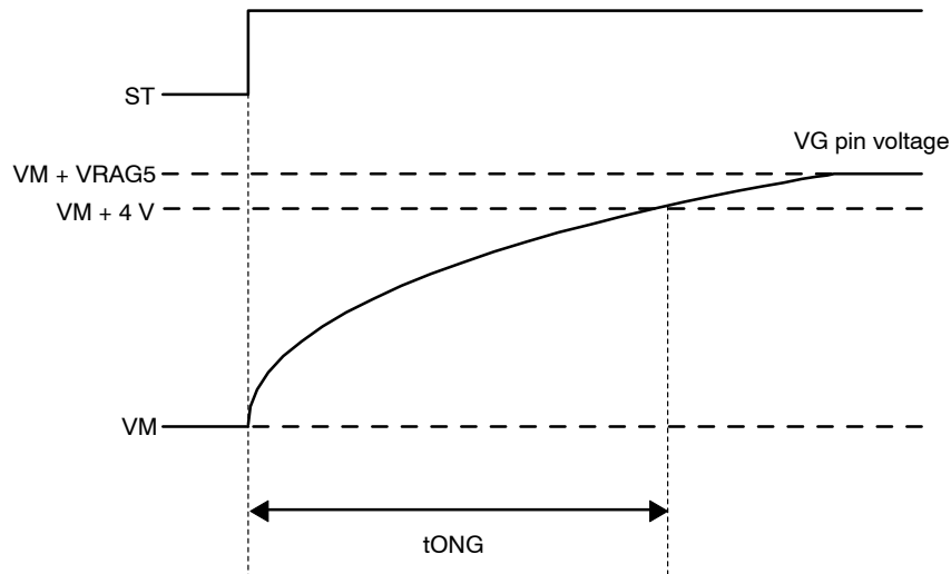
Figure 21. VG Pin Voltage Schematic View
