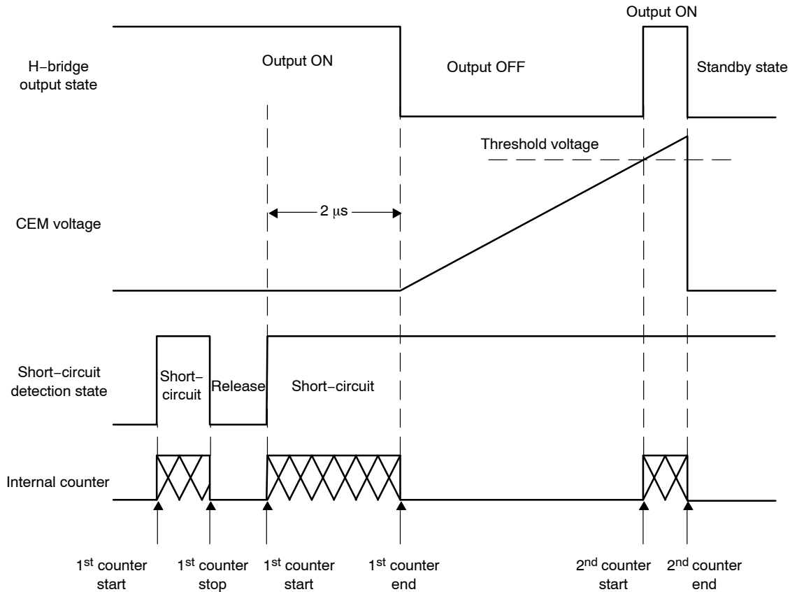
Figure 20. Latch Type
