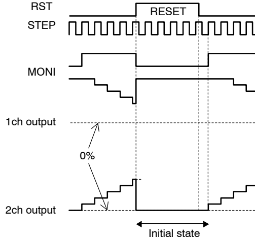
Figure 7. Reset Function
