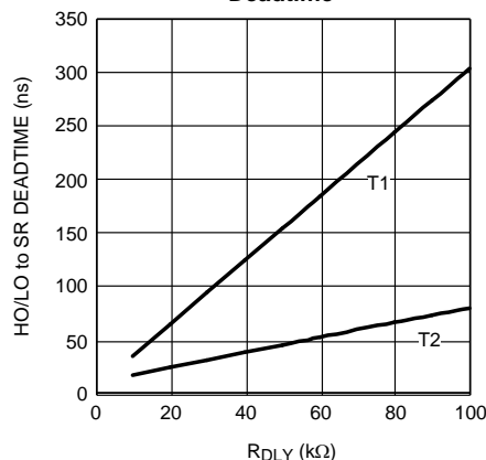
R_{\text{DLY}} vs Deadtime
