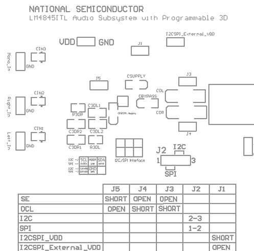
Figure 73. Top Overlay
