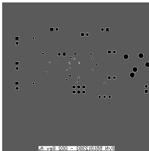
Figure 75. Bottom Layer
