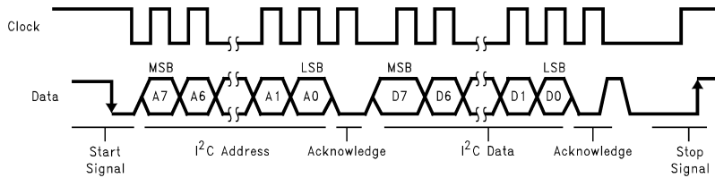
Figure 68. I²C Bus Format
