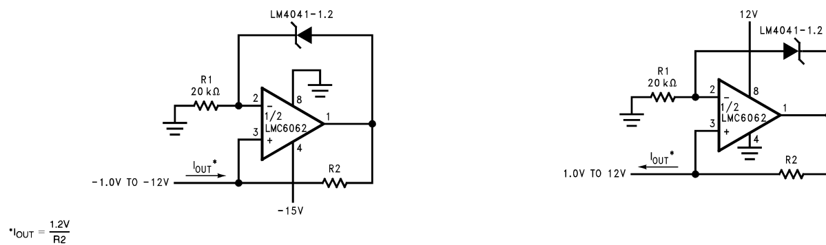
Figure 32. Precision 1 µA to 1 mA Current Sources
