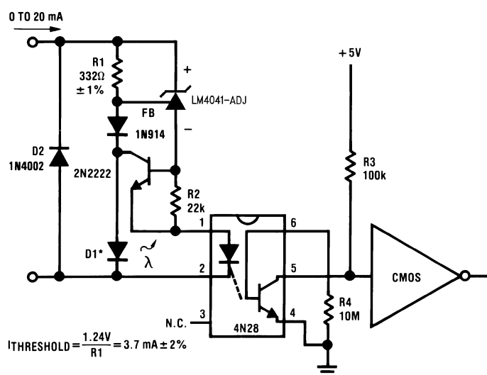
Figure 31. Precision Floating Current Detector
