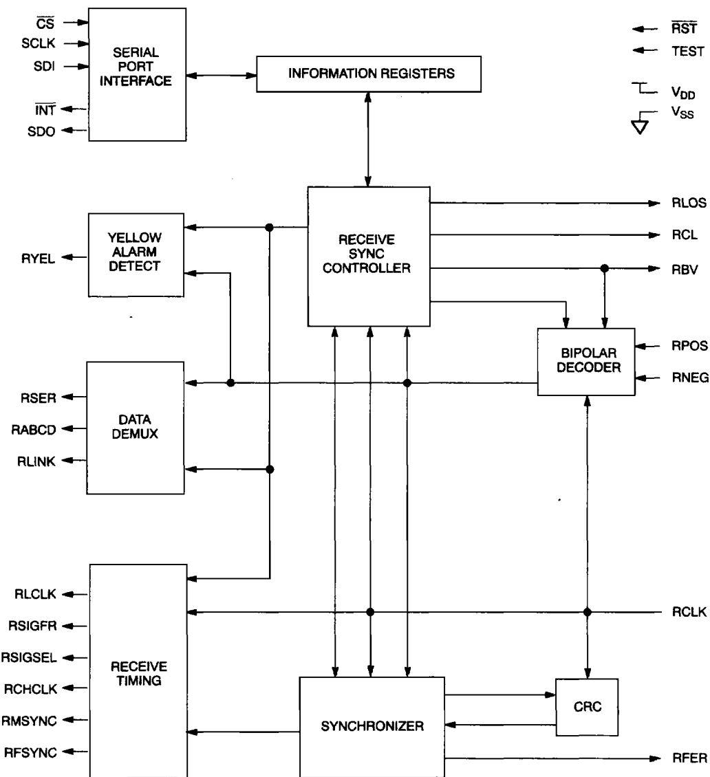
DS2182 BLOCK DIAGRAM Figure 1
