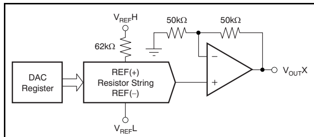
Figure 92. DAC8165 Architecture
