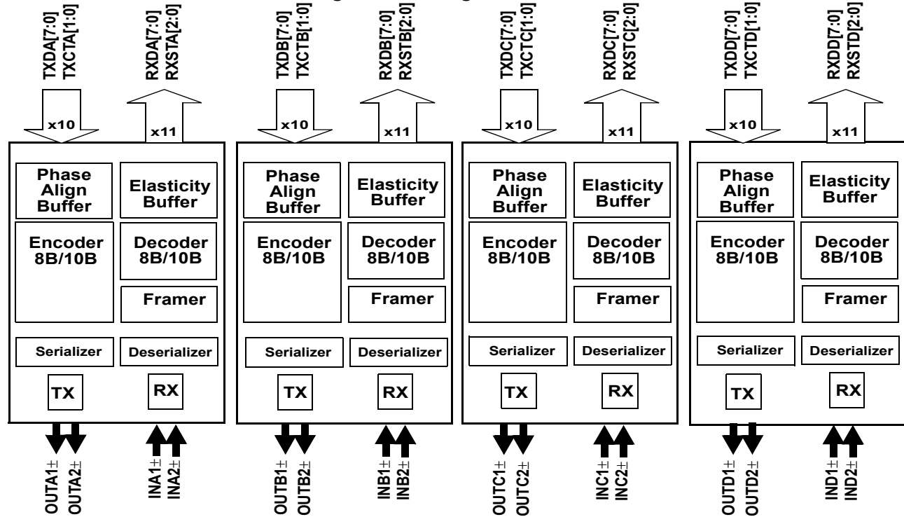
CYP(V)(W)15G0401DXB Transceiver Logic Block Diagram
