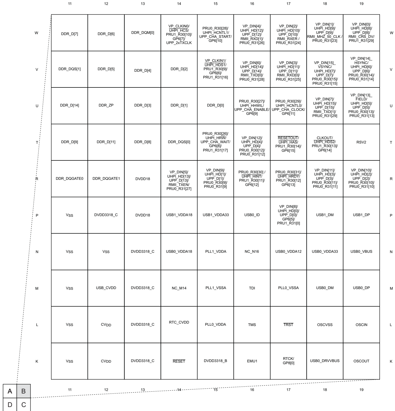
Figure 3-2. Pin Map (Quad B)
