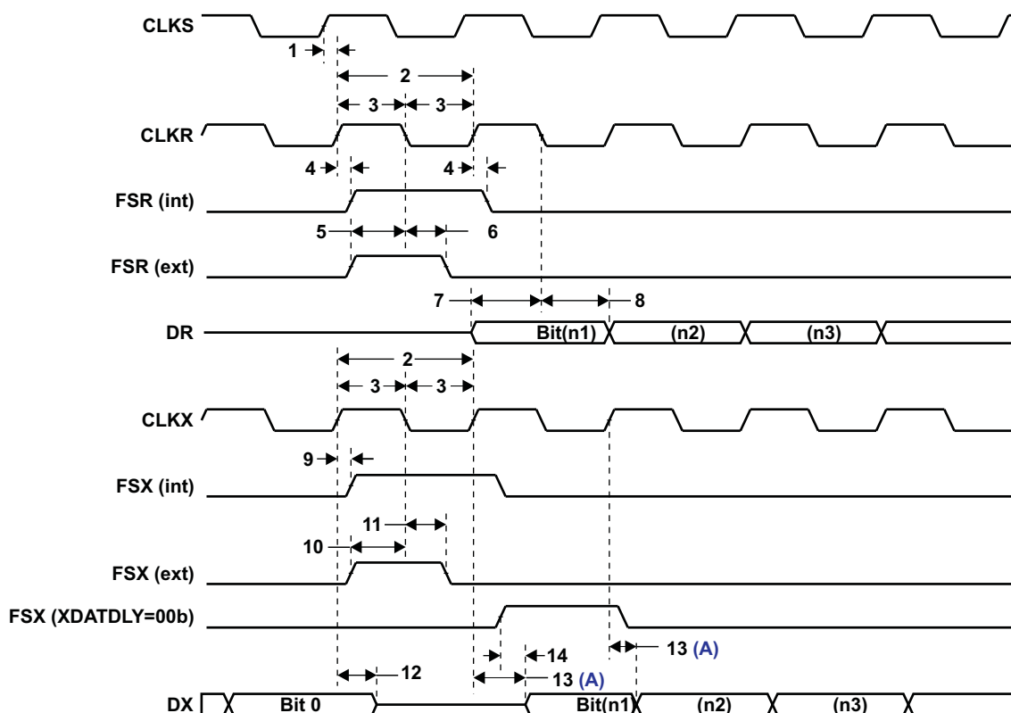
Figure 6-32. McBSP Timing
