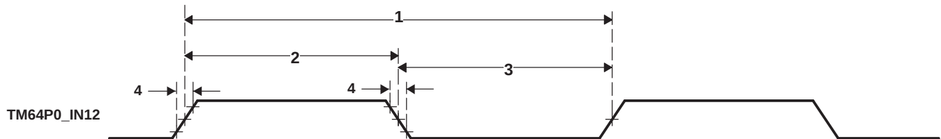
Figure 6-80. Timer Timing
