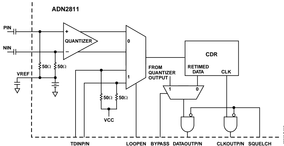
Figure 18. Test Modes
